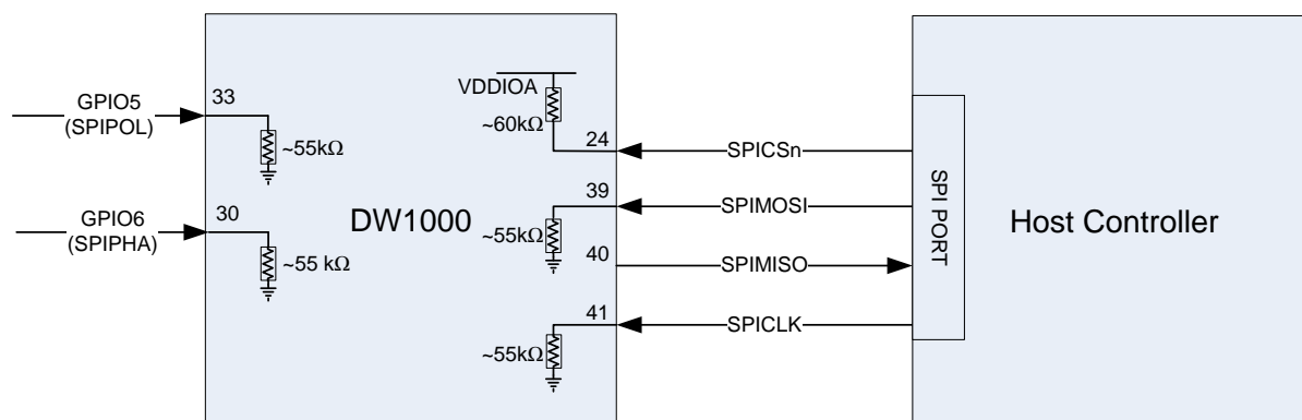
Figure 25: SPI Connections
