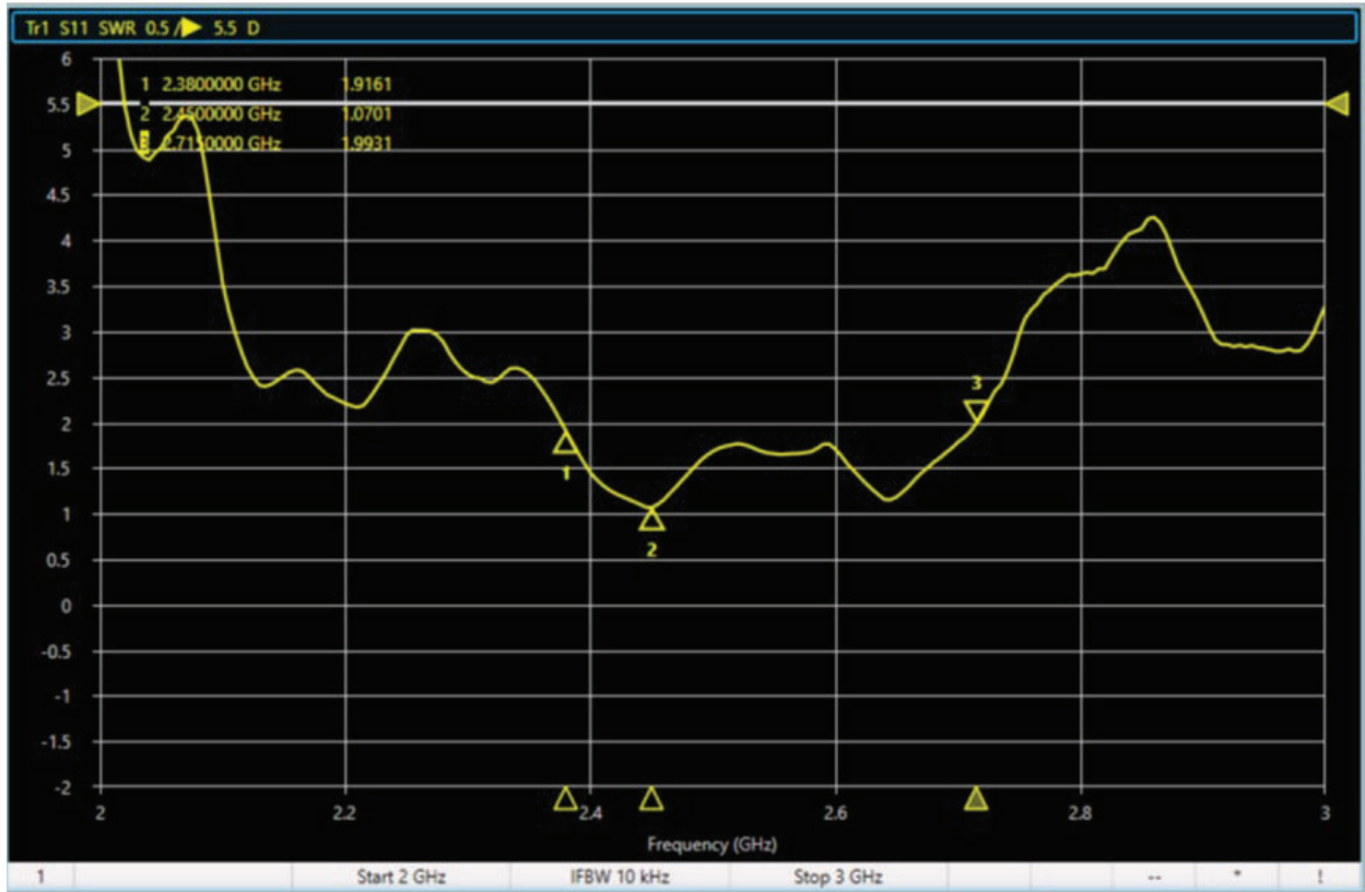
SWR diagram of the IFA Antenna for the RF Remote Control Remoter
